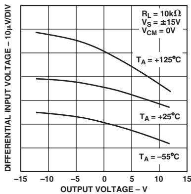
Figure 16. Open-Loop Gain Linearity
